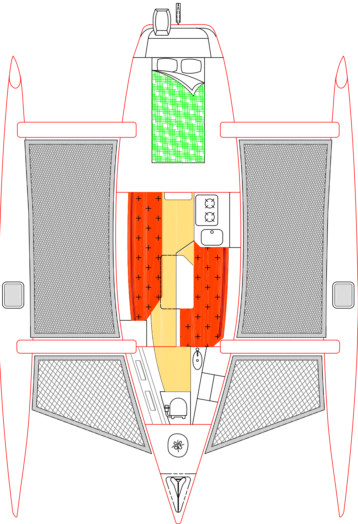
- ACCOMMODATION PLAN - CORSAIR 31UC ULTIMATE CRUISER
