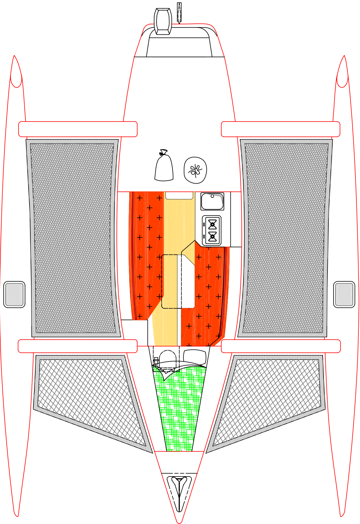
- ACCOMMODATION PLAN - CORSAIR 31RS AFT COCKPIT
